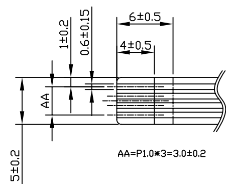
DETAIL A (Scale=3/2)
